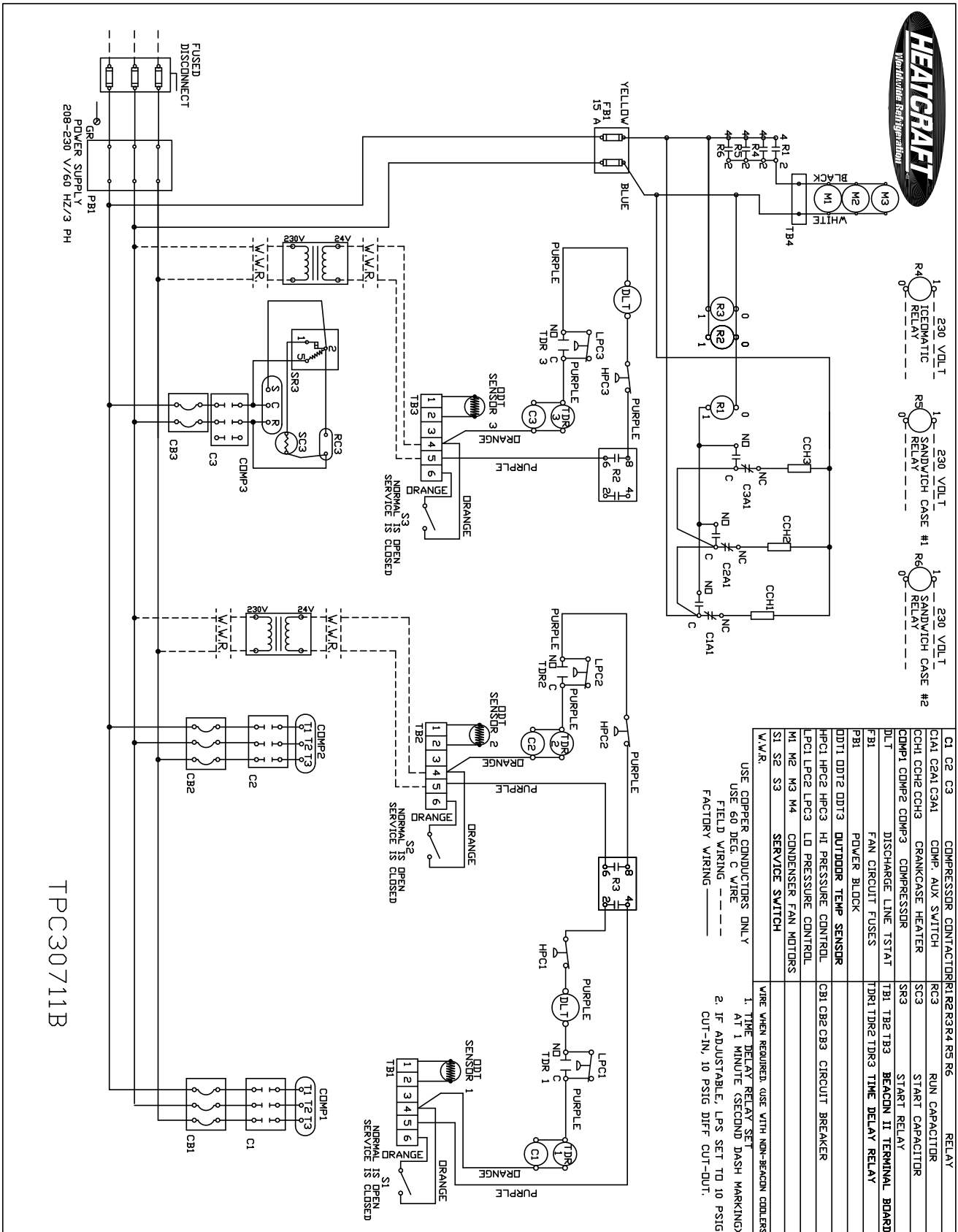
Diagram 4. Typical Wiring Diagram
