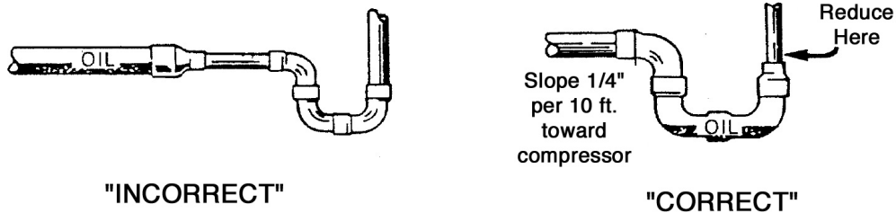
Figure 4. Suction P-traps
