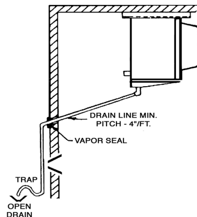
Figure 5. Drain Line
