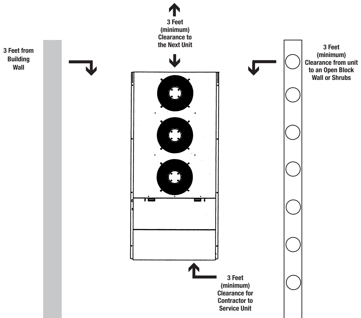
Figure 2. Condensing Unit Placement
