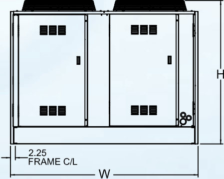
Unit Diagram 4
