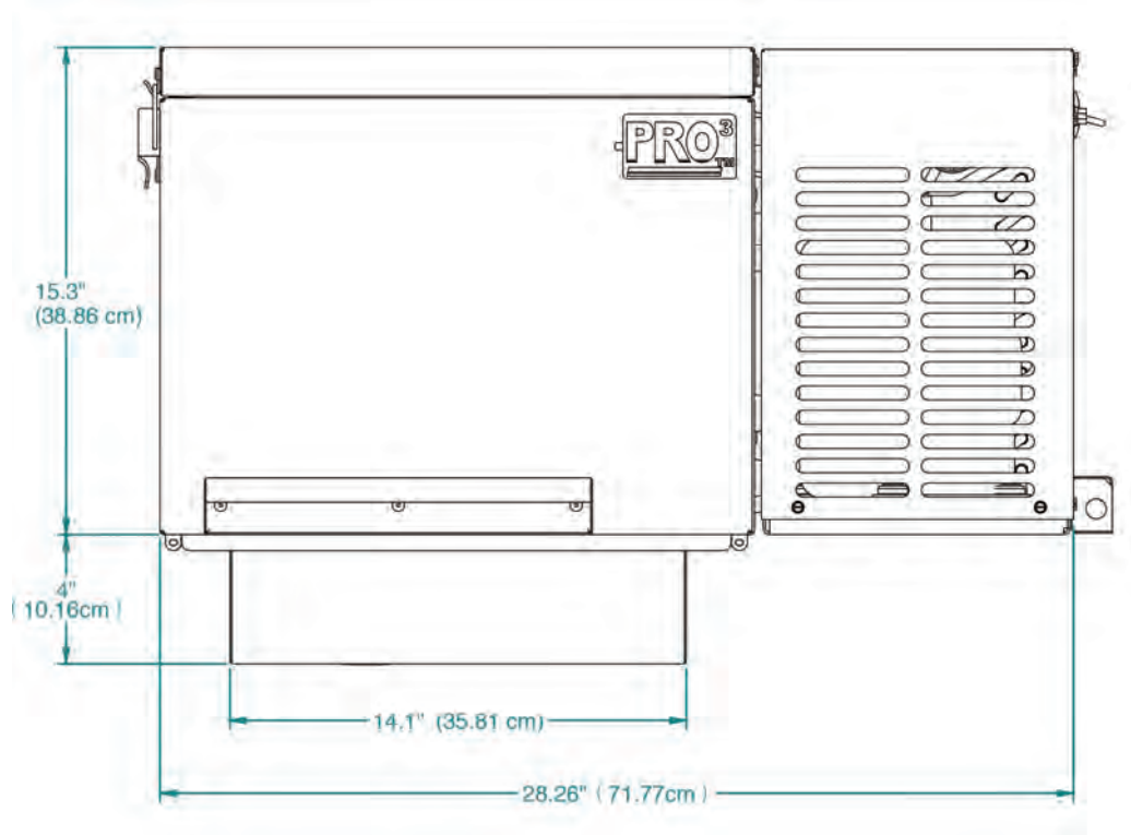
FIGURE 1 P1 CABINET DESIGN/INDOOR ONLY
