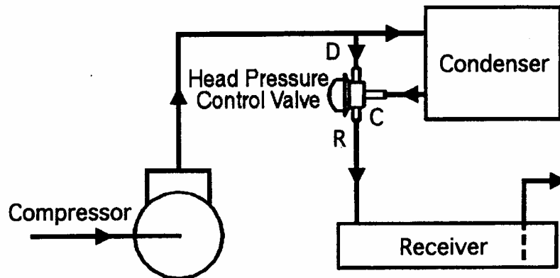
Figure 1. Single Valve Flooded System
