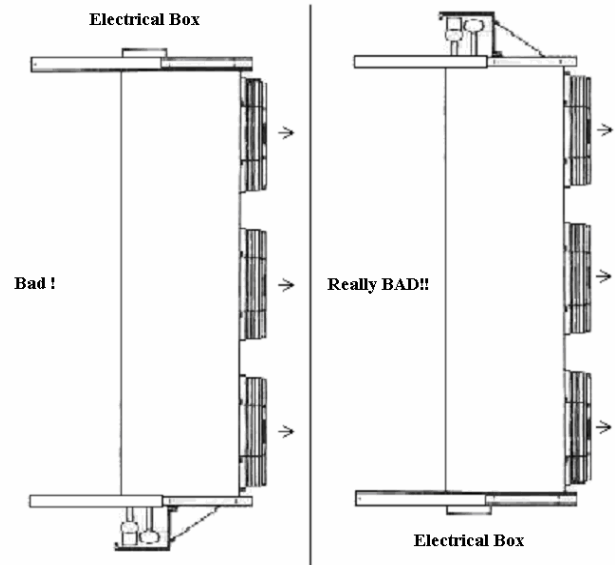
Fig. 2: Improper orientation
